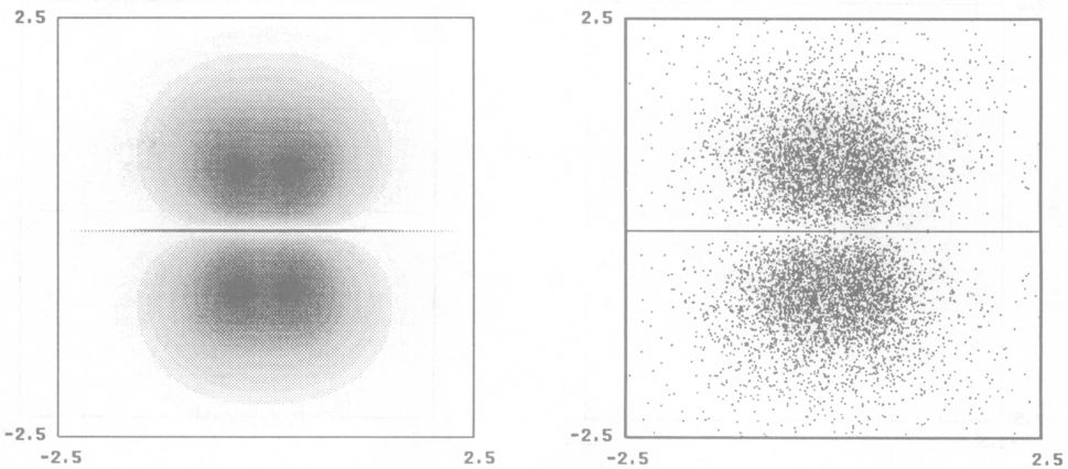
FIGURE 2. Random cubics ( n = 4 ). Note that, for the left-hand plots, the grey-scales for h_n and g_n are produced separately and in such a way that both use the full range from white to black.
