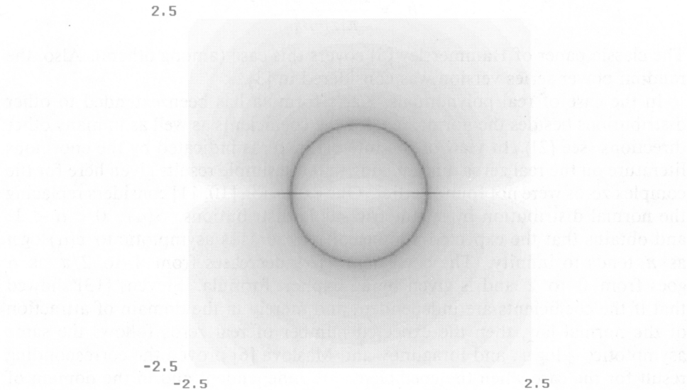
FIGURE 6. Limiting intensity (using a logarithmic grey-scale).
