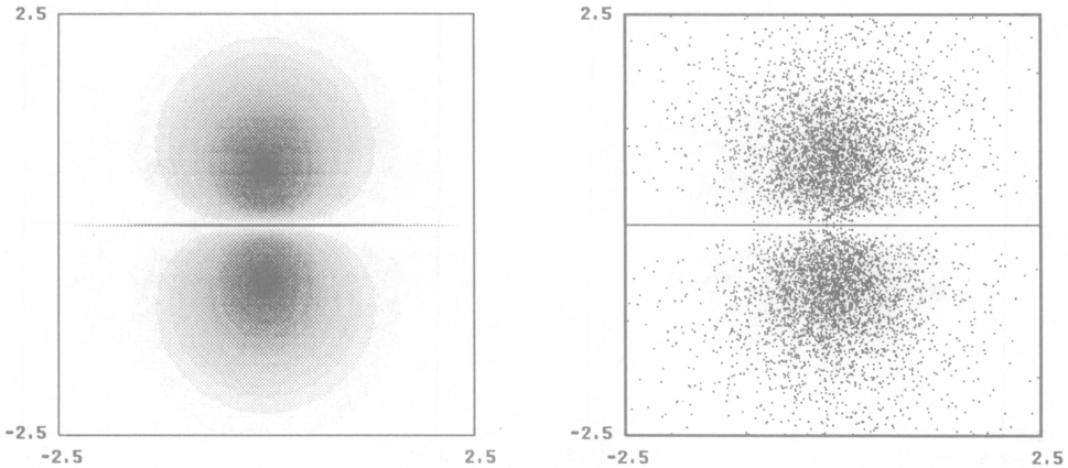
FIGURE 1. Random quadratics ( n = 3 ). In this figure and the next several, the left-hand plot is a grey-scale image of the intensity functions h_n and g_n (which is concentrated on the x -axis). The right-hand plot shows 20,000 roots from randomly generated polynomials. Subsequent captions give more information pertaining to each of these figures.
